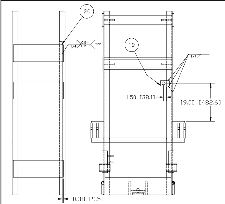
REAR VIEW OF K3606 INNER RAIL REAR VIEW OF K3606 OUTER RAIL
